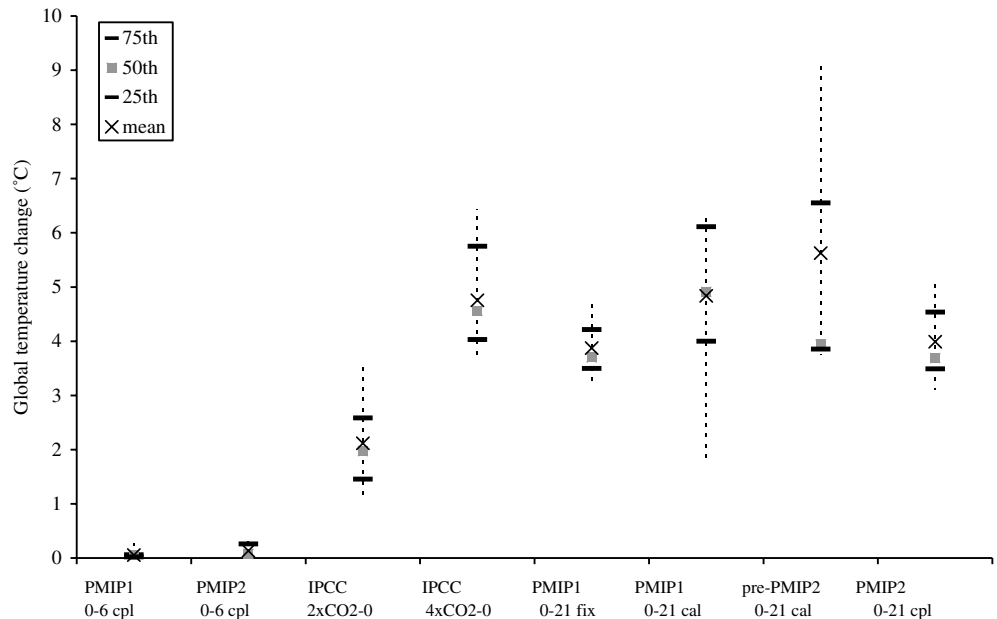
Fig. 2 Annual mean global temperature changes simulated by a variety of climate models run under similar boundary conditions. The full range (dashed line), mean (cross symbol), 25th (lower bold dash symbol), 50th (grey square symbol), 75th (upper bold dash symbol) percentiles of the various model results are calculated from the distribution of the various model results (see Table 2). The “fix”, “slab” and “cpl” abbreviations refer to different configurations of models used and are described in Sect. 3 and Table 1
