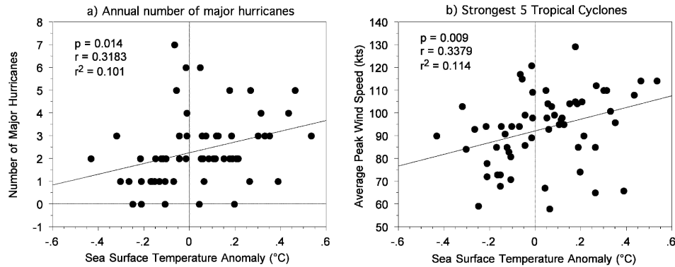
FIG. 1. Scatterplots showing the observed relationship between SSTs and two measures of hurricane intensity: (a) the number of major hurricanes (tropical cyclones of category 3, 4, or 5 on the Saffir–Simpson hurricane scale) each year and (b) the average peak wind speed in the five strongest storms in each year, for the period 1944 to 2002 in the Atlantic basin.
