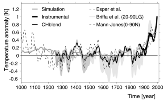
Figure 2: Reconstructions of Northern Hemisphere temperatures over the past millennium from “proxy” observations (primarily tree-ring records) from various sources (grey bands, thin lines, and dotted lines), compared with instrumental observations (thick black line) and a simulation using a simple
