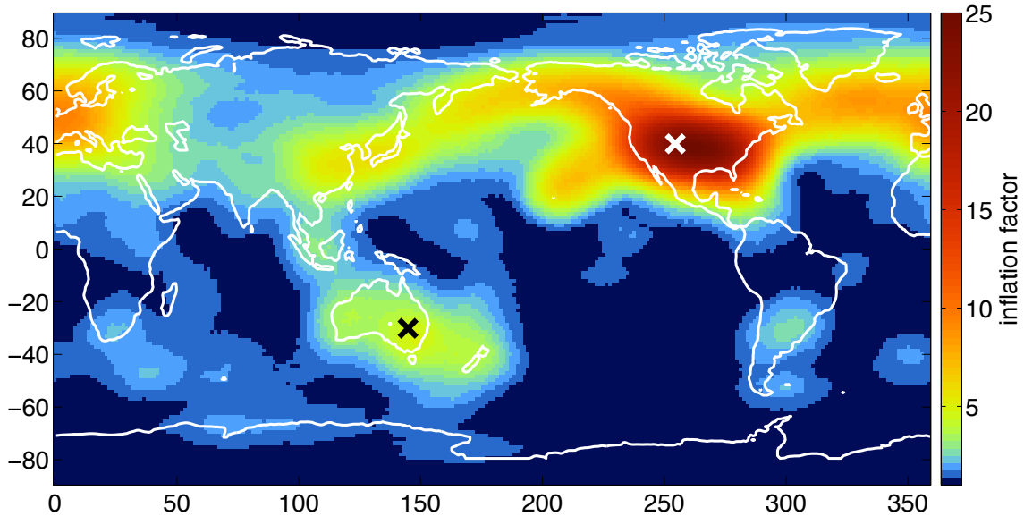
Figure 3: The field of spatial inflation values, \lambda , at the end of the assimilation period.
