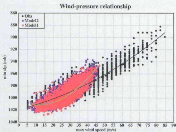
FIG. 4. Scatterplot of maximum surface wind speed ( m\ s^{-1} ) versus minimum central surface pressure (hPa) for observed (black) and simulated (red = Model1; blue = Model2) Atlantic TCs (1980–2006). Model1 data are for 1980–2005. Solid lines are least squares quadratic best-fit lines to the points.
