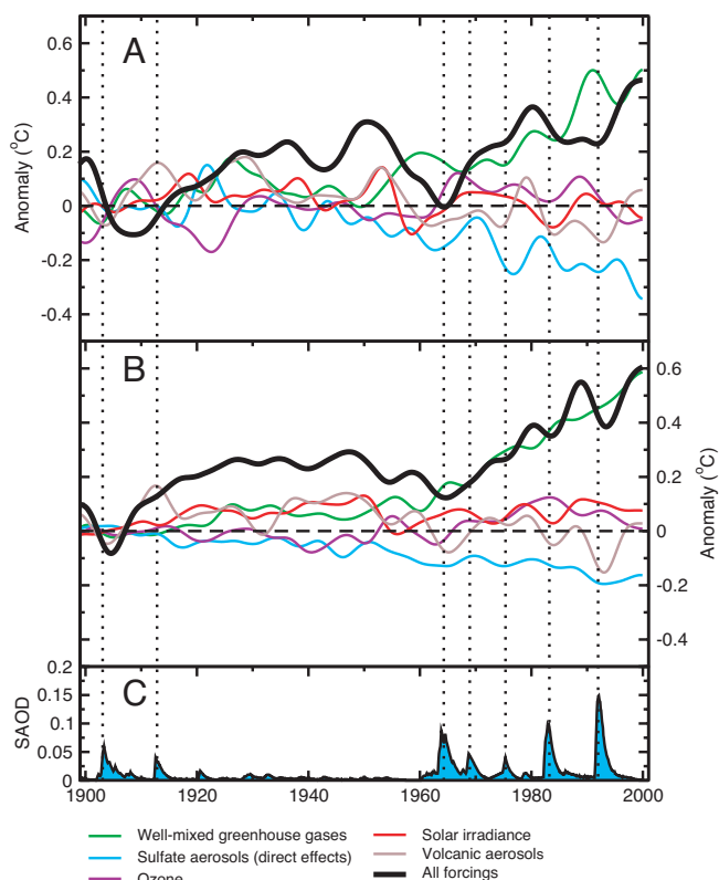
Fig. 5. Contribution of different external forcings to SST changes in tropical cyclone regions. (A and B) Results are for the ACR (A) and PCR (B) and are from a 20CEN run and single-forcing experiments performed with the PCM (27). Each result is the low-pass filtered average of a four-member ensemble, with window width W = 145 months. For anomaly definition, refer to Fig. 1. Stratospheric aerosol optical depth (21) is also shown (C).
